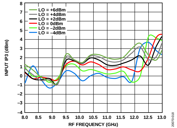
Figure 19. Input IP3 vs. RF Frequency at Various LO Powers, T_A = 25^\circ\text{C}
