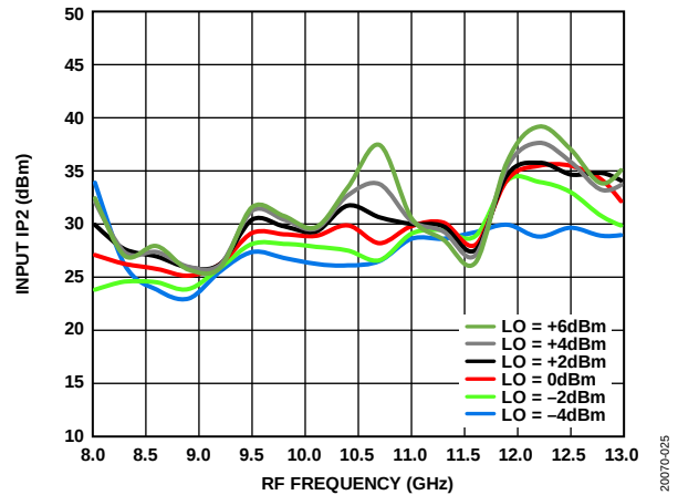
Figure 26. Input IP2 vs. RF Frequency at Various LO Powers, T_A = 25^\circ\text{C}
