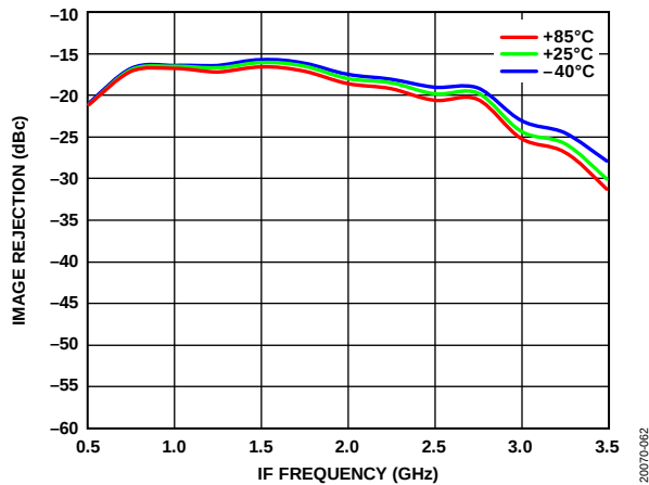
Figure 63. Image Rejection vs. IF Frequency at Various Temperatures
