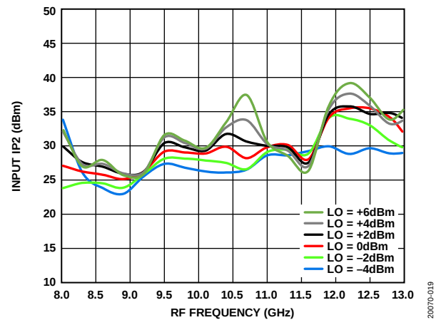
Figure 20. Input IP2 vs. RF Frequency at Various LO Powers, T_A = 25^\circ\text{C}
