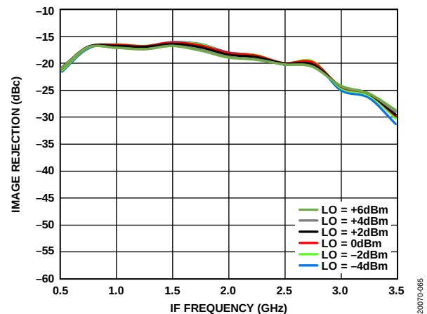
Figure 66. Image Rejection vs. IF Frequency at Various LO Powers, T_A = 25^\circ\text{C}
