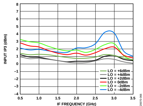
Figure 67. Input IP3 vs. IF Frequency at Various LO Powers, T_A = 25^\circ\text{C}
