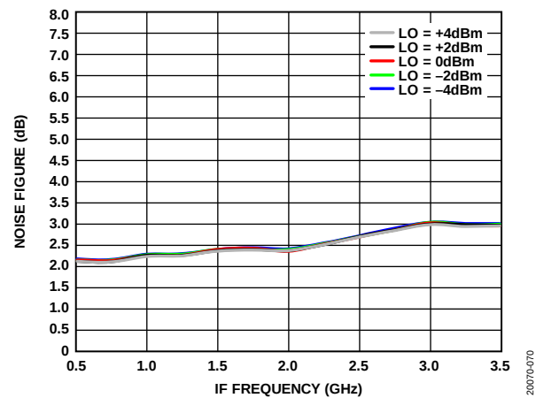
Figure 71. Noise Figure vs. IF Frequency at Various LO Powers, TA = 25°C
