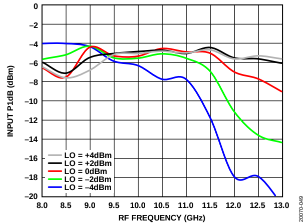
Figure 50. Input P1dB vs. RF Frequency at Various LO Powers, T_A = 25^\circ\text{C}
