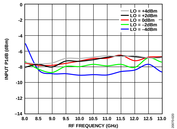
Figure 21. Input P1dB vs. RF Frequency at Various LO Powers, T_A = 25^\circ\text{C}
