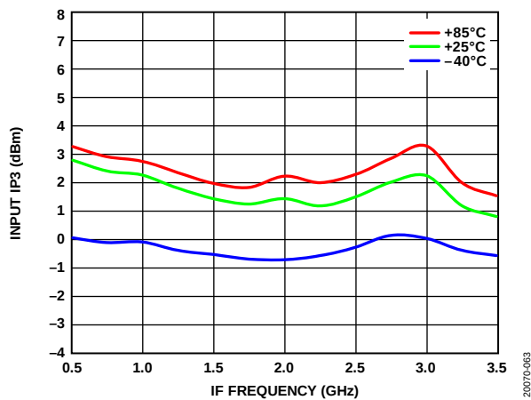
Figure 64. Input IP3 vs. IF Frequency at Various Temperatures
