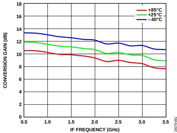
Figure 62. Conversion Gain vs. IF Frequency at Various Temperatures
