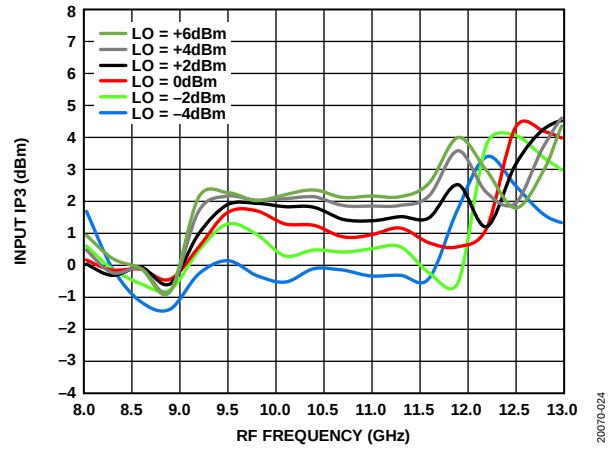
Figure 25. Input IP3 vs. RF Frequency at Various LO Powers, T_A = 25^\circ\text{C}
