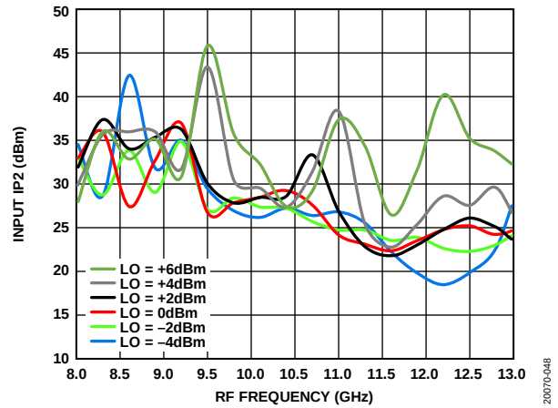
Figure 49. Input IP2 vs. RF Frequency at Various LO Powers, T_A = 25^\circ\text{C}
