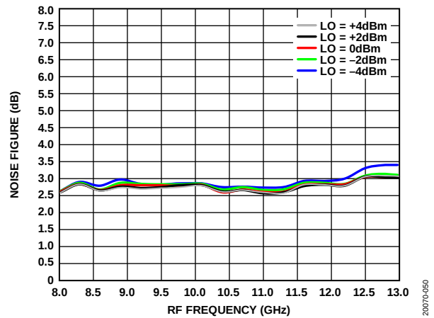
Figure 51. Noise Figure vs. RF Frequency at Various LO Powers, T_A = 25^\circ\text{C}
