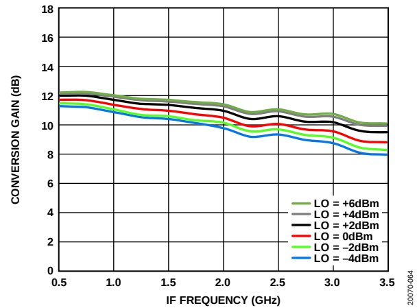
Figure 65. Conversion Gain vs. IF Frequency at Various LO Powers, T_A = 25^\circ\text{C}
