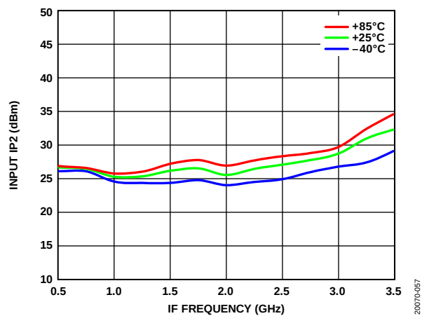
Figure 58. Input IP2 vs. IF Frequency at Various Temperatures
