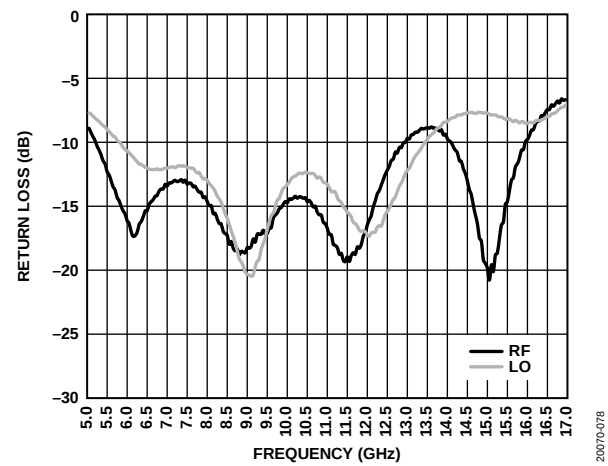
Figure 79. Return Loss vs. Frequency, LO = 0 dBm at 10 GHz, T_A = 25^\circ\text{C}
