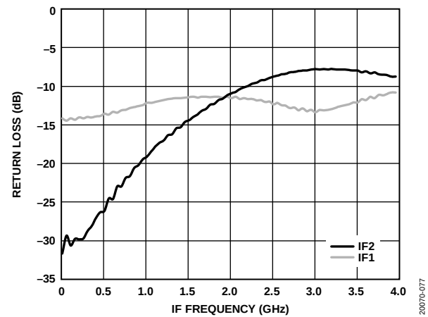
Figure 78. Return Loss vs. IF Frequency, LO = 17 dBm, T_A = 25^\circ\text{C}
