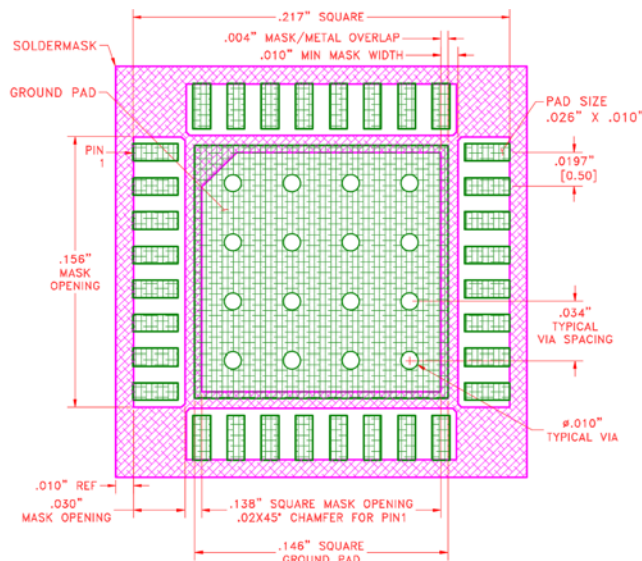
Figure 80. PCB Land Pattern Footprint of the EV1HMC908ALC5
