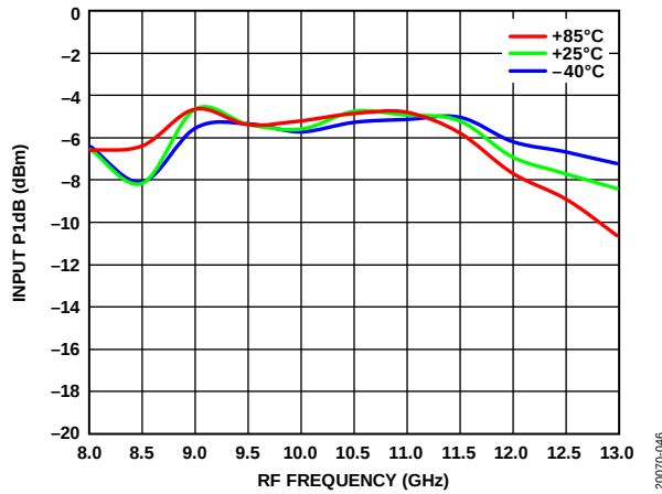
Figure 47. Input P1dB vs. RF Frequency at Various Temperatures
